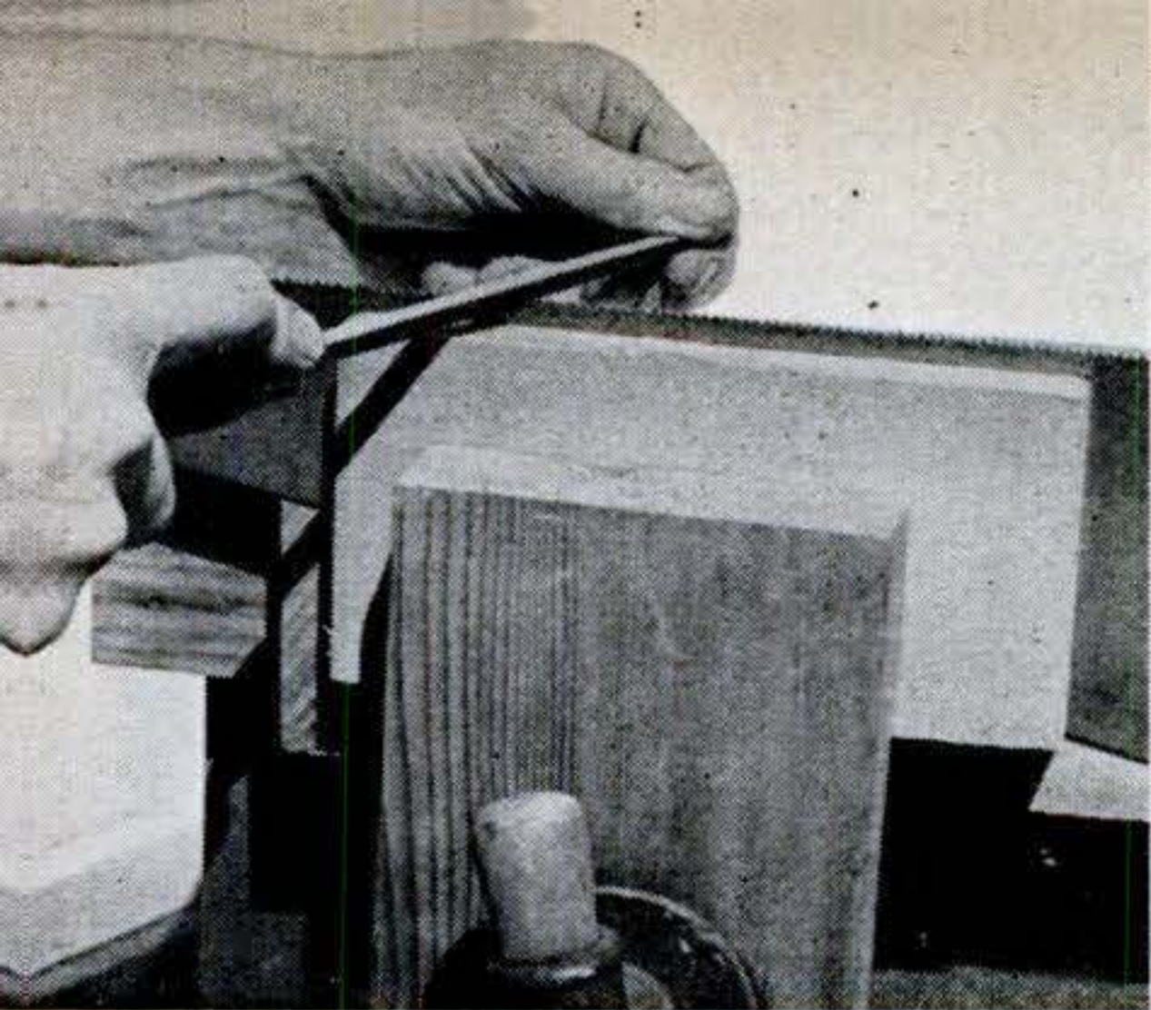
A SLIM TAPER FILE at work sharpening a saw. Two blocks of wood are used in a bench vise to clamp the saw in the absence of a special saw vise.
